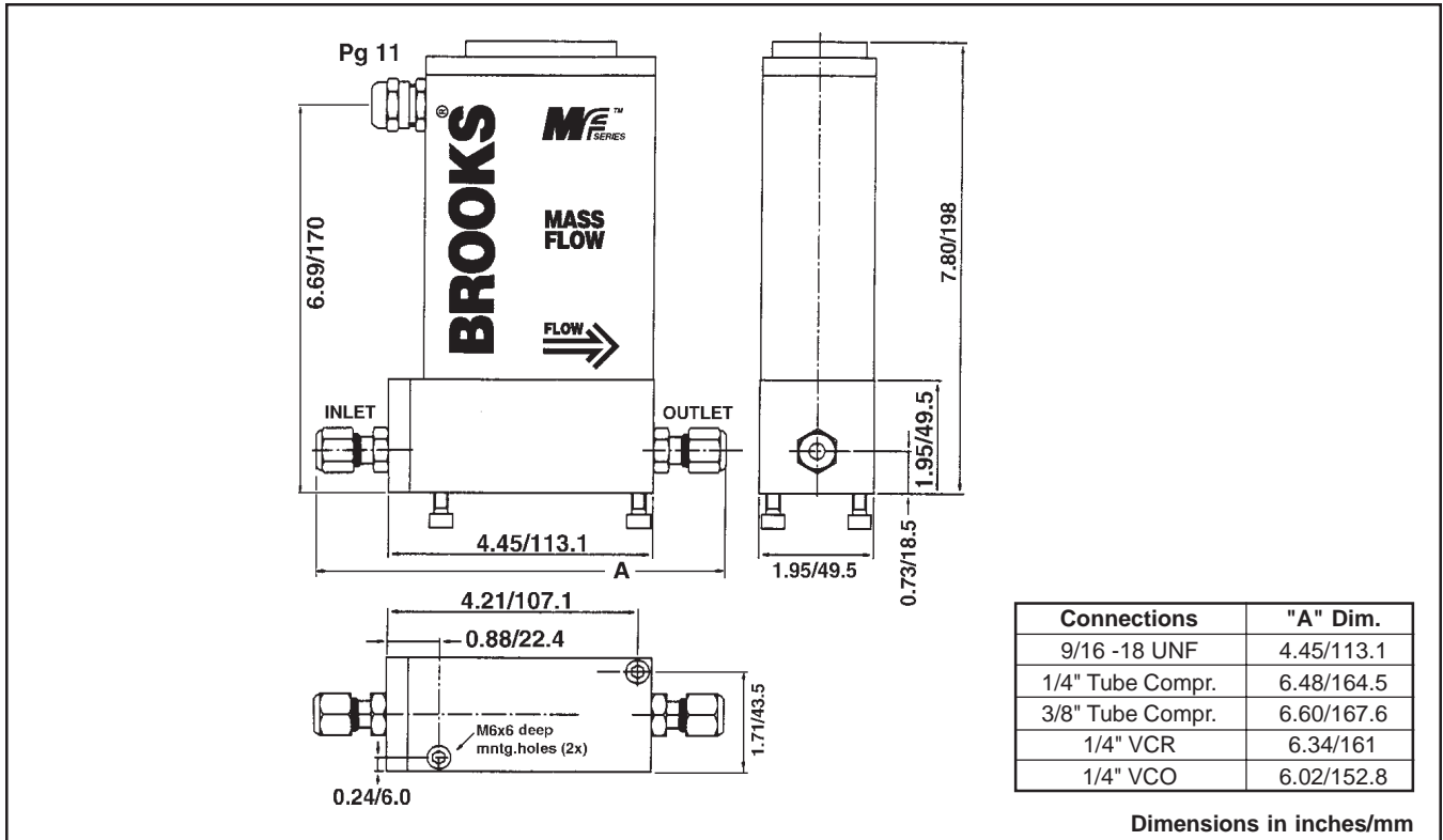
Figure 9 Model Mf61 Meter Dimensions
