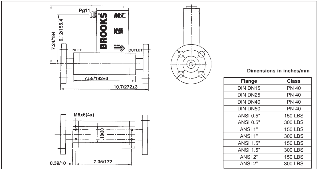
Figure 11 Model Mf63 Meter with Flange Dimensions
