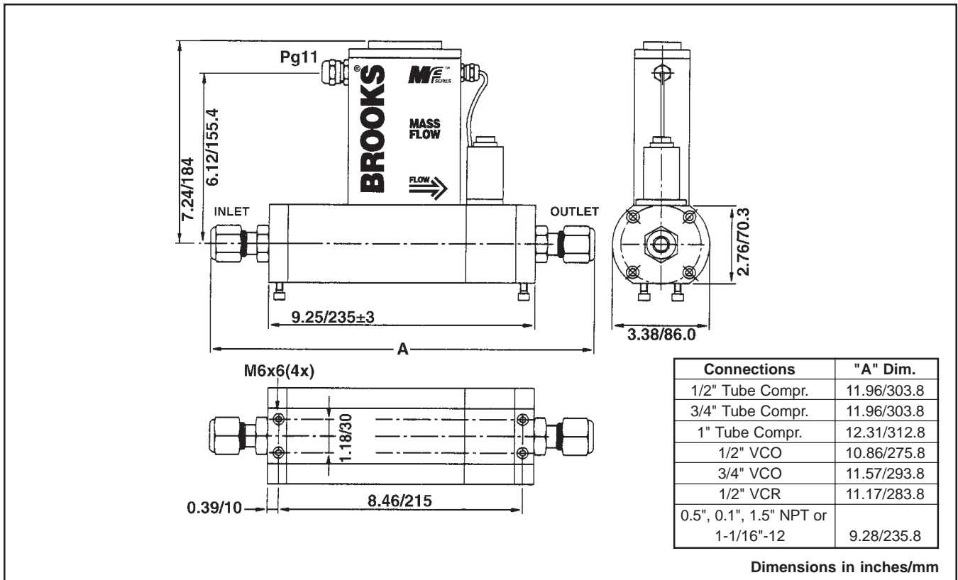
Figure 6 Model Mf53 Controller Dimensions
